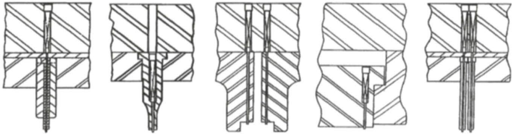
NARROW PUNCH IN SPLIT QUILL
